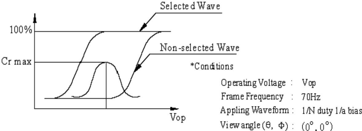
Note 4: Definition of contrast ratio.( Test LCD using DMS501)
